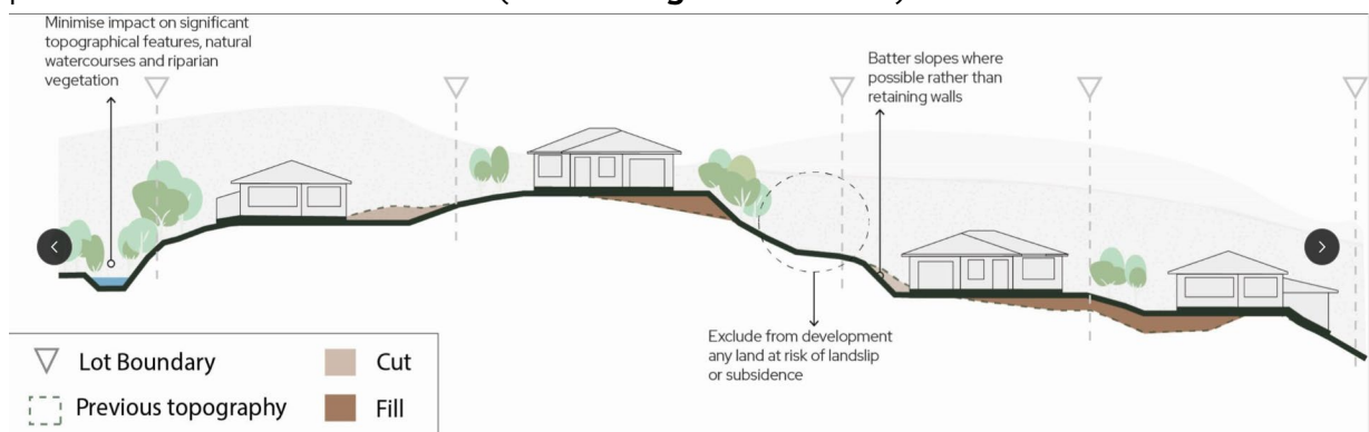
Figure C.5: Alterations to natural landform minimising the overall scale of earthworks
