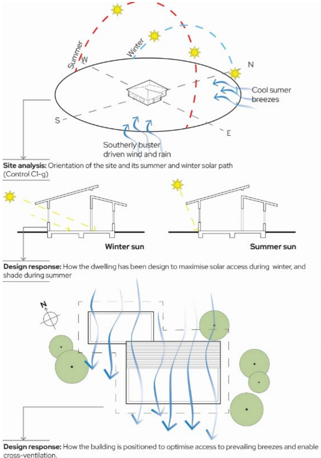
Figure D1.3: Principles of passive design to be addressed by the site analysis and design response plan
