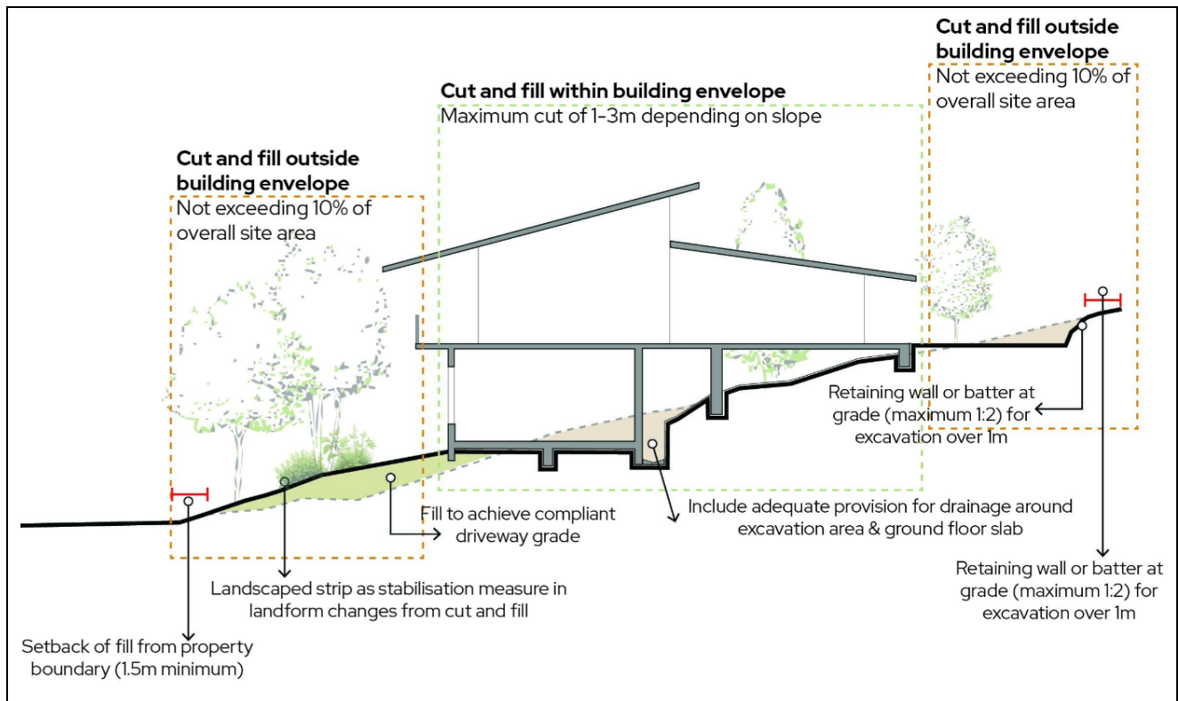
Figure D1.6: The key elements required to establish slope-responsive design
