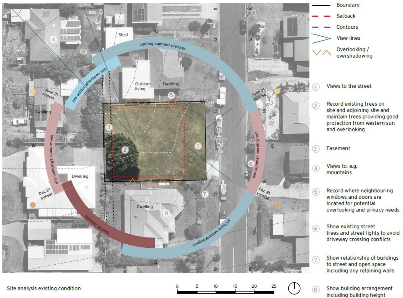
Figure D1.1: Example site analysis plan
