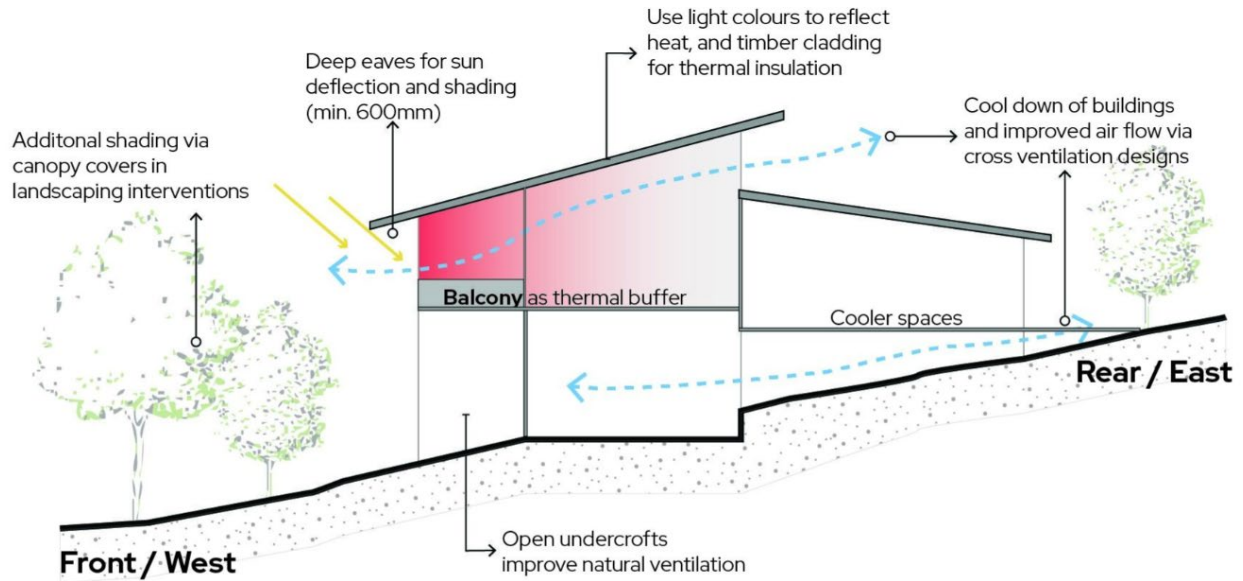
Figure D1.8: How building design & materiality contributes to passive design principles
